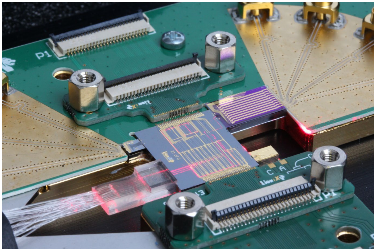
Figure 2: RF-Beamformer assembly featuring a large PIC with SiN waveguides, and butt-coupled integration of an InP modulator array (top right), InP gain chip (bottom right) and InP array of photodetectors (top-left). © LioniX International BV
