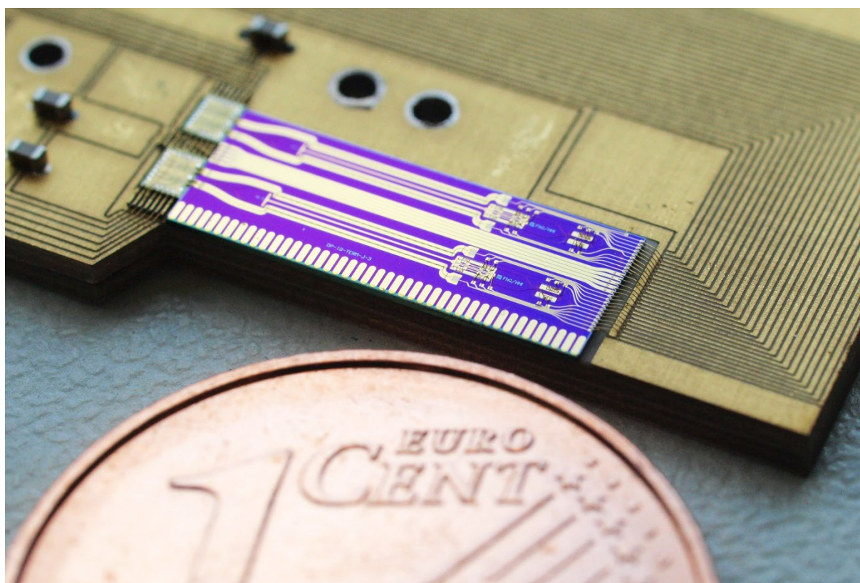
Figure 1: Dual Polarisation IQ Modulator for 512 Gbit/s transmission with 16QAM, and coin for scale. © Fraunhofer HHI
